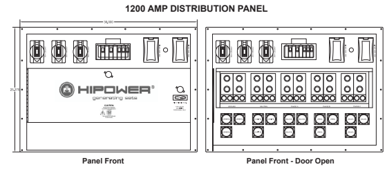
Pictures of Control Panel (Top photo) and Distribution Panel may include optional equipment and/or accessories
